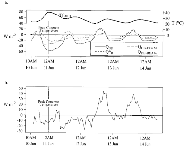
FIG. 12. (a) Hourly averaged bottom surface energy balance for the 1999 bridge: Q_{H-BEAM} is the amount of heat transferred vertically through the beam by conduction; Q_{H-FORM} is the amount of heat transferred vertically through the form. The heavy dashed line is the temperature of the bottom surface of the form ( T_{form} ). (b) Measured heat transferred from between the beams to the ambient environment.
