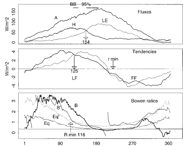
FIG. 2. (top) Daily averaged fluxes above the canopy at Harvard Forest for 1991–98. Available energy A = (-Q^* - Q_g) , sensible heat flux H , and latent heat flux LE (dotted). Here “BB” and “95%” are as indicated in Fig. 1, and H = LE at day 154. (center) 1946–94 daily averaged and smoothed temperature tendency ( C_p \partial T / \partial t , solid) and humidity tendency ( L \partial q / \partial t , dotted). Tendencies are equal at day 125. Here “r min” represents the average date of the annual minimum canopy resistance at Harvard Forest (Sakai et al. 1997). Here “LF” and “FF” represent climatological last and first 0^\circ\text{C} freeze dates. (bottom) Bowen ratios B and B' and equilibrium Bowen ratios Eq' and Eq as described in the text. Date of average annual minimum relative humidity “R min 116” indicated.
